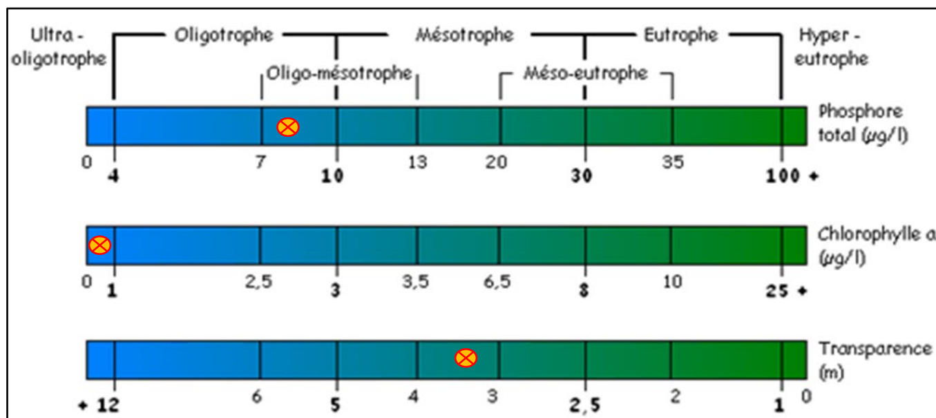
Figure 8 – État trophique 2025 – Station 1 – Lac Corrigan (C1)
