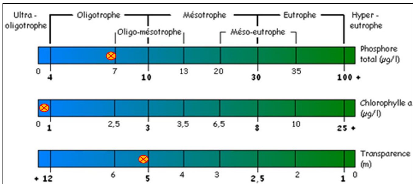
Figure 13 – État trophique 2025 – Station 1 – Lac Dame (DA1)
