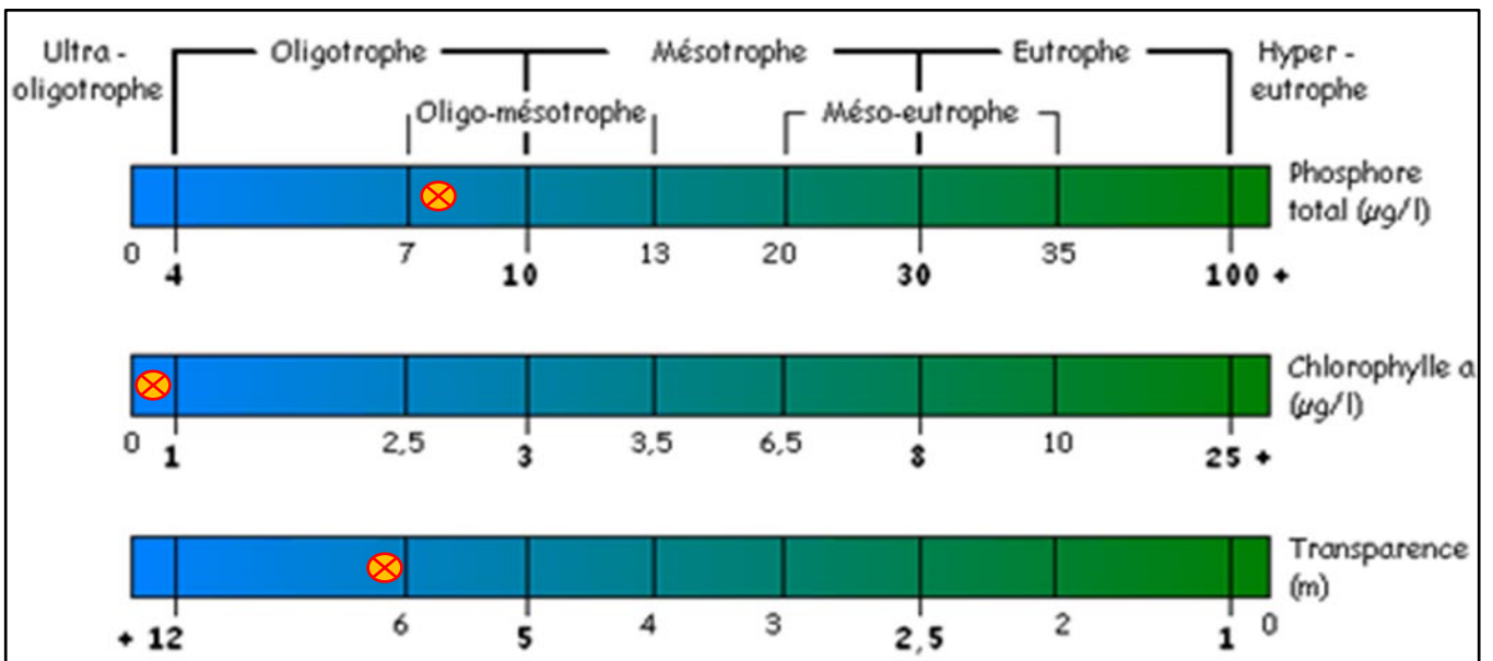
Figure 17 – État trophique 2025 – Station 3 – Lac Grand (G3)
