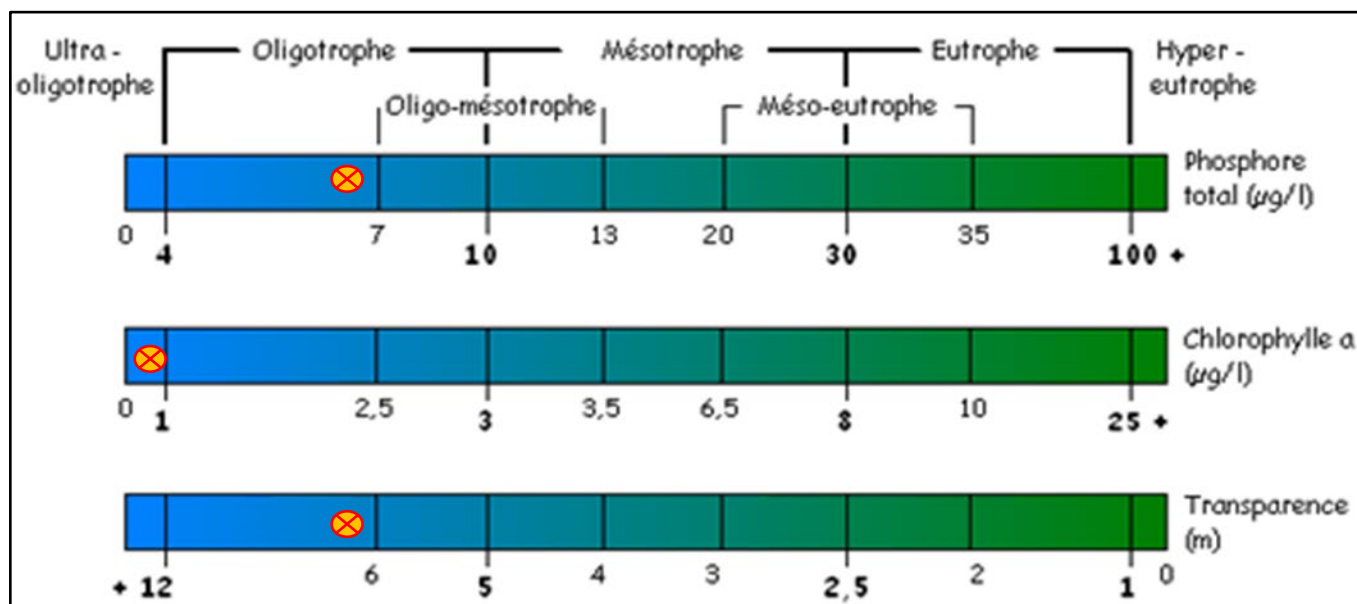
Figure 15 – État trophique 2025 – Station 1 – Lac Grand (G1)
