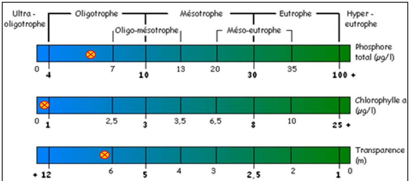
Figure 16 – État trophique 2025 – Station 2 – Lac Grand (G2)
