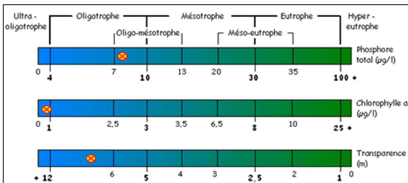
Figure 12 – État trophique 2025 – Station 1 – Lac McGlashan (MGA1)
