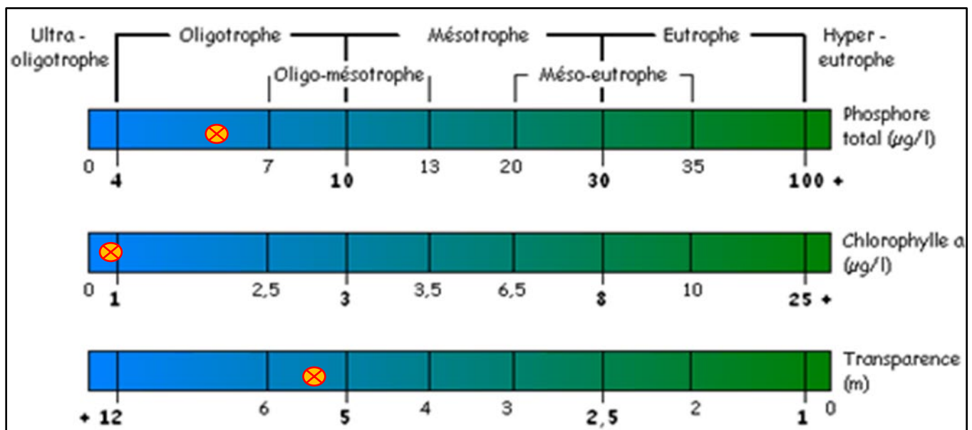
Figure 15 – État trophique 2025 – Station 1 – Lac McGregor (MG1)
