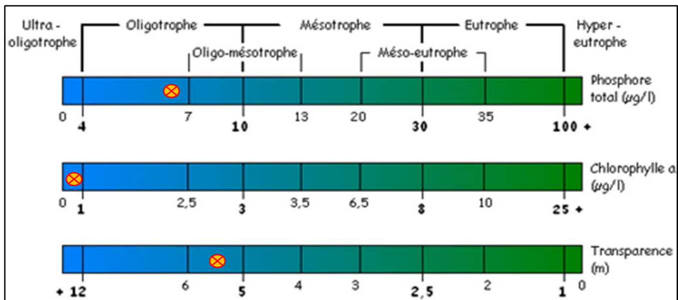
Figure 16 – État trophique 2025 – Station 2 – Lac McGregor (MG2)
