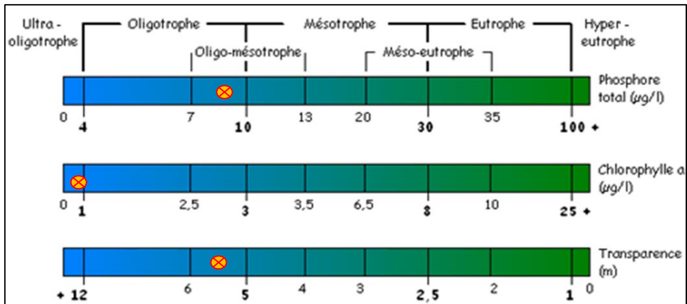
Figure 17 – État trophique 2025 – Station 3 – Lac McGregor (MG3)
