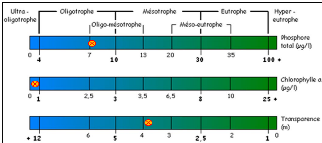
Figure 17 – État trophique 2025 – Station 3 – Lac Saint-Germain (SG3)
